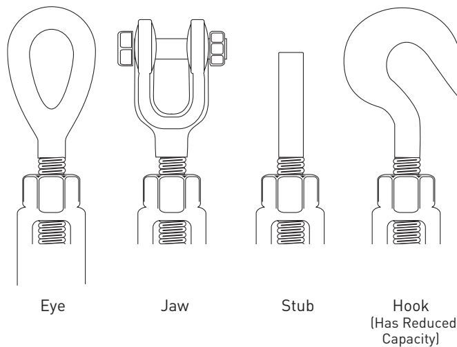
Turnbuckle End Fittings
